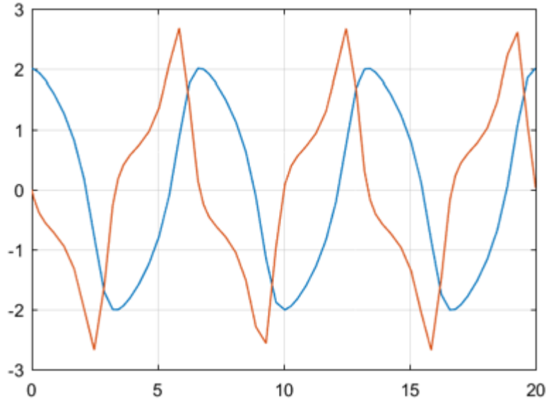
The van der Pol Equation results from my model:
