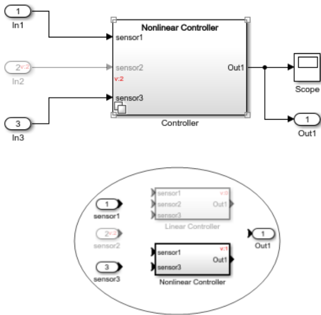
Components of 'Controller' block
